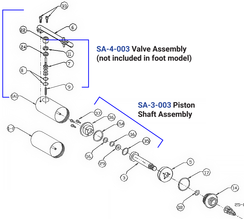
SA-1-003 Piston Housing Assembly
